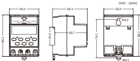
Outline and installation hole size (or 35mm standard guide rail installation)
